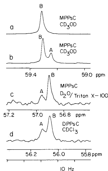
FIGURE 7: ^{31}\text{P} NMR spectra of MPPsC: (a) pure MPPsC(B) in \text{CD}_3\text{OD} ; (b) MPPsC (B/A \approx 3/1, \text{CD}_3\text{OD} ); (c) same as (b), in \text{D}_2\text{O} plus 5% Triton X-100; (d) after reacylation to DPPsC (B/A \approx 3/1, \text{CDCl}_3 ). Sample concentration was 10 mM. Spectral parameters were the same as in Figure 3. Temperature was 37 °C (a-c) and 30 °C (d).
