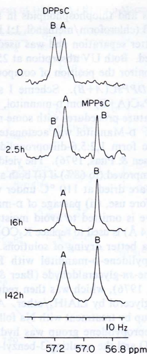
FIGURE 3: Stereospecific hydrolysis of DPPsC(B) by bee venom phospholipase A_2 followed by ^{31}\text{P} NMR. Sample conditions: 20\ \mu\text{mol} of DPPsC(A+B) in 2 mL of buffer containing 50 mM Mops-Na, pH 7.2, 0.25 mM EDTA, 35% \text{D}_2\text{O} , 5% Triton X-100, 2.5 mM puratronic grade \text{Ca}(\text{NO}_3)_2 , and 3.8\ \mu\text{g} of PL A_2 from bee venom. NMR parameters: spectral width 1000 Hz; acquisition time 4.1 s; pulse width 12\ \mu\text{s} ; ^1\text{H} decoupling; line broadening -1\ \text{Hz} ; Gaussian broadening 0.05 Hz. The probe temperature was set at 37^\circ\text{C} , and the sample was incubated at 37^\circ\text{C} .
