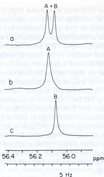
FIGURE 1: ^{31}\text{P} NMR spectra of DPPsC (10 mM in \text{CDCl}_3 ). (a) Mixture of diastereomers from chemical synthesis; (b) pure isomer A recovered from hydrolysis by phospholipase A_2 ; (c) pure isomer B obtained from acylation of the product of phospholipase A_2 hydrolysis, MPPsC(B). NMR parameters: spectral width 1000 Hz; acquisition time 4.1 s; ^1\text{H} decoupling; line broadening 0.1 Hz; pulse width 12\ \mu\text{s} ( 90^\circ pulse at 20\ \mu\text{s} ); temperature 30^\circ\text{C} .
